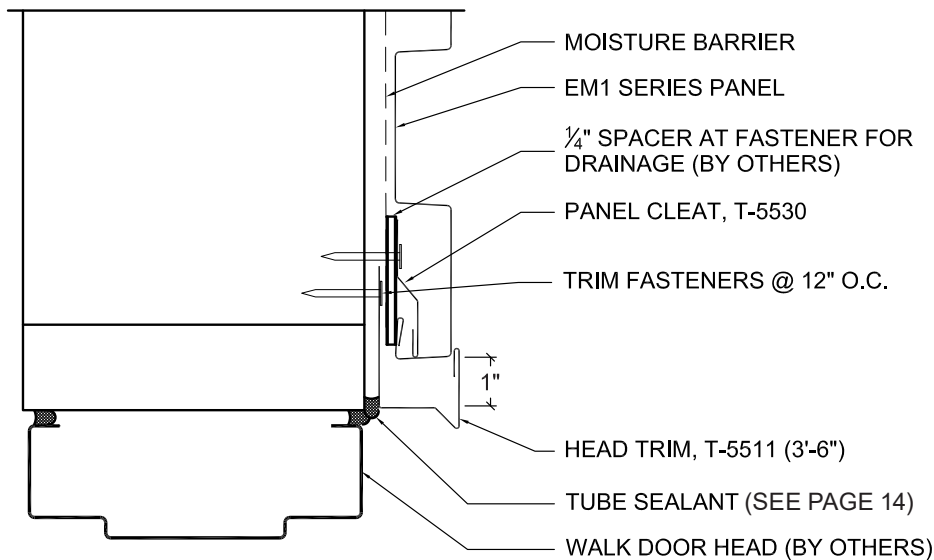
ELEVATION VIEW
